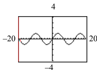
Zoom Trigonometry
